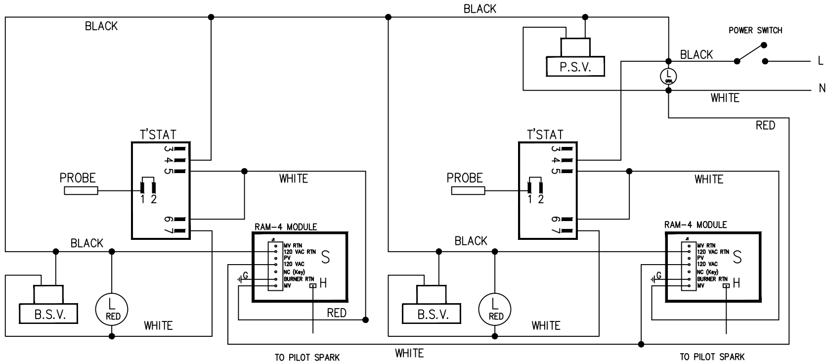
WIRING DIAGRAM FOR ONE THERMOSTAT OPERATING ONE BURNER
