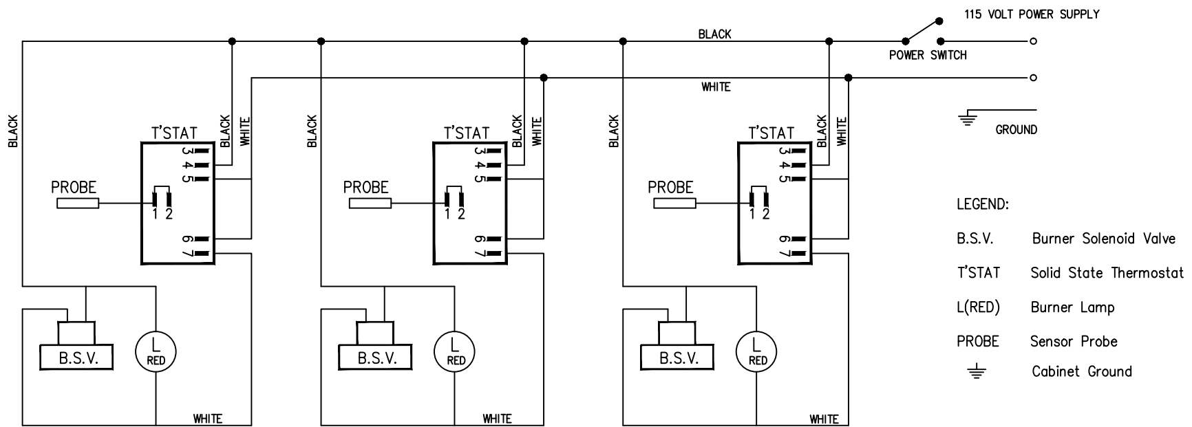
WIRING DIAGRAM FOR ONE THERMOSTAT OPERATING ONE BURNER
